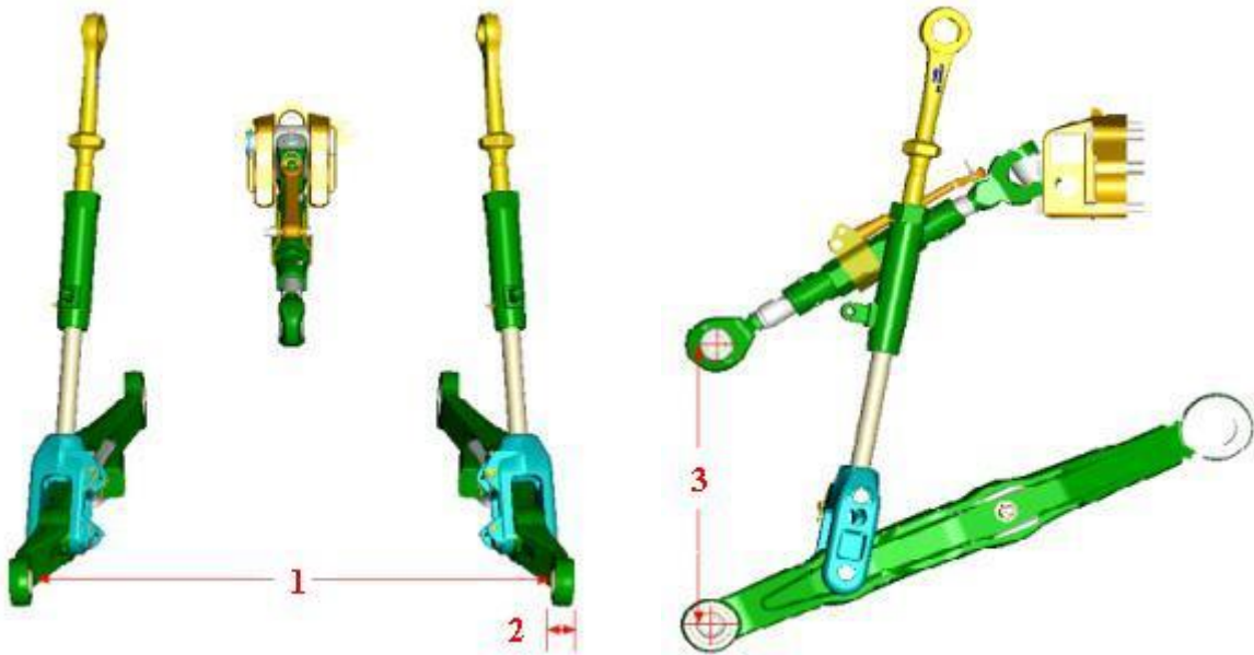
3-point hitch (1) (2)
